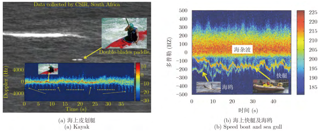
图6 典型海上微动目标回波特性 Fig. 6 Properties of some typical marine targets with micromotion
