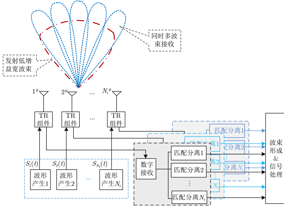
图1 集中式MIMO雷达收发结构 Fig. 1 Collected MIMO radar transceiver structure
