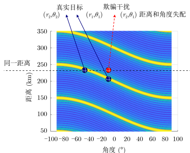
图3 LFM步进频频分MIMO雷达发射功率距离-角度耦合 Fig. 3 Distance-angle coupling of LFM stepped frequency division MIMO radar transmit power
